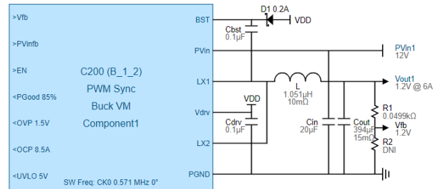
Example Schematic symbol for Power Components
