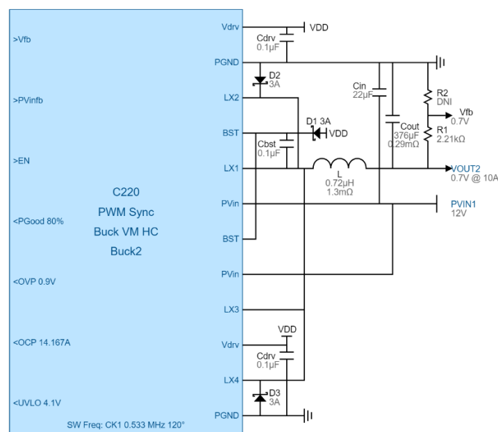
Figure 6b. Buck, 10A Typical WebAmP Schematic
