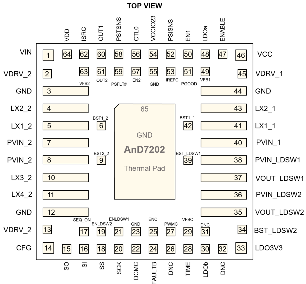
Figure 2. AnD7202 package pinout
