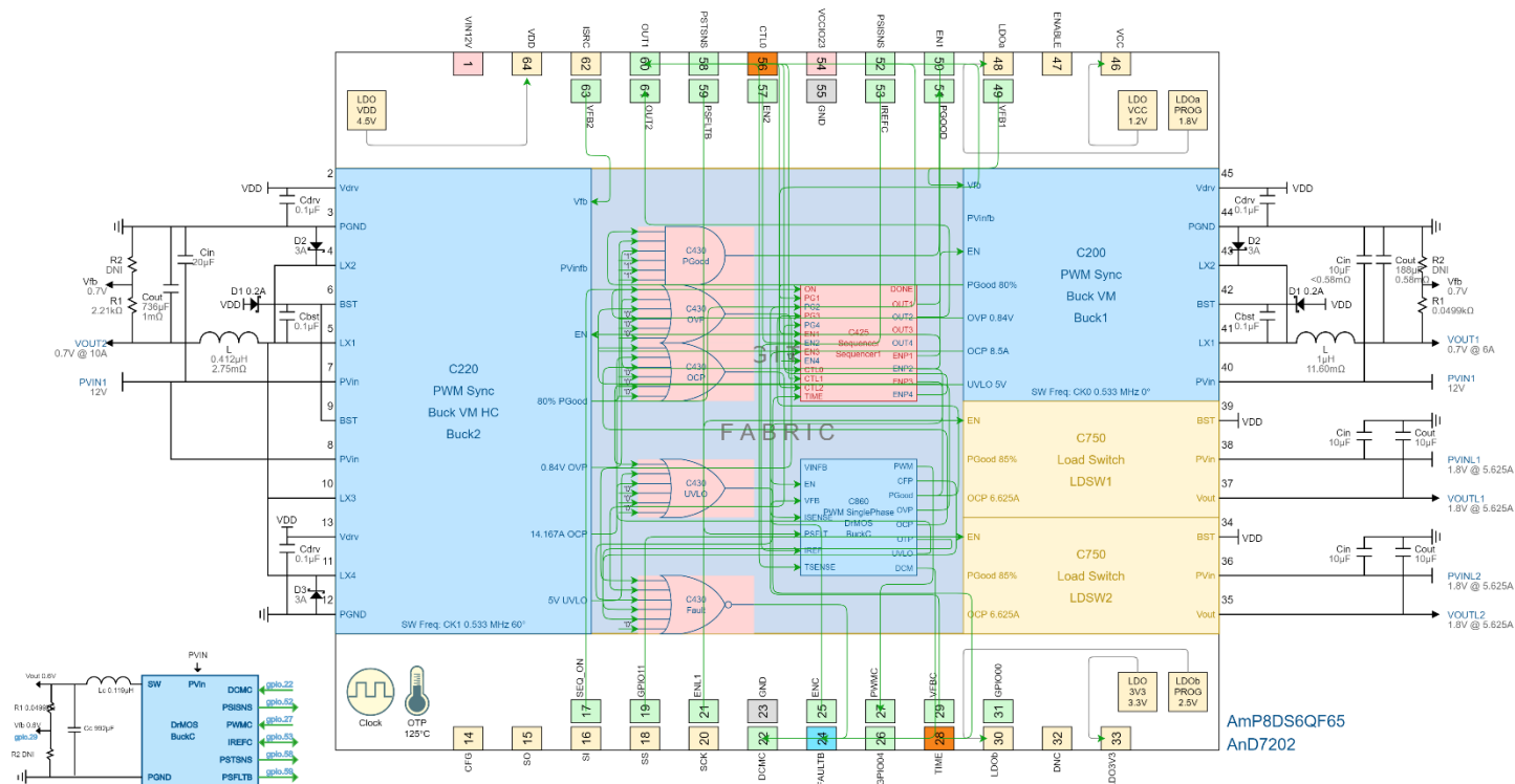
Figure 1. AnD7202 WebAmP Design View
