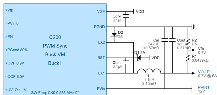
Figure 6a: Buck1, 6A Typical WebAmP Schematic
