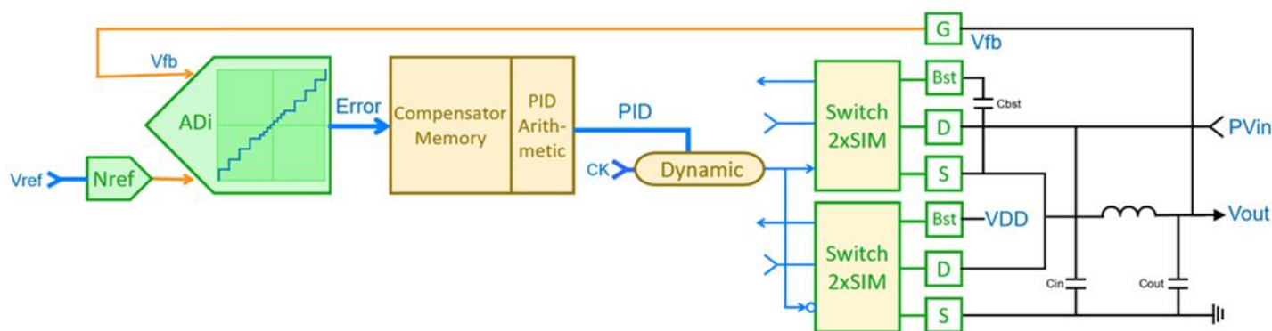
Figure 13: PMIC Blocks and Resources Example - Buck Regulator
