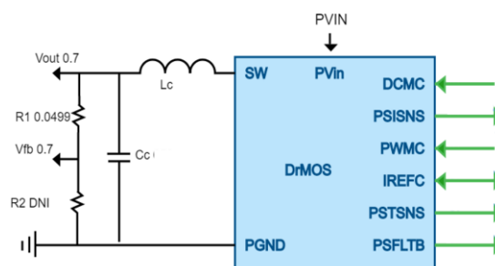
Figure 4. AnD7202 interface with DrMOS
