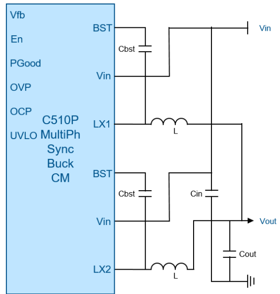
Figure 1: C510 application schematic (two phases shown)
