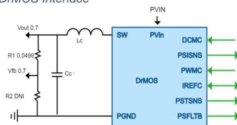
Figure 2: DrMOS Interface
