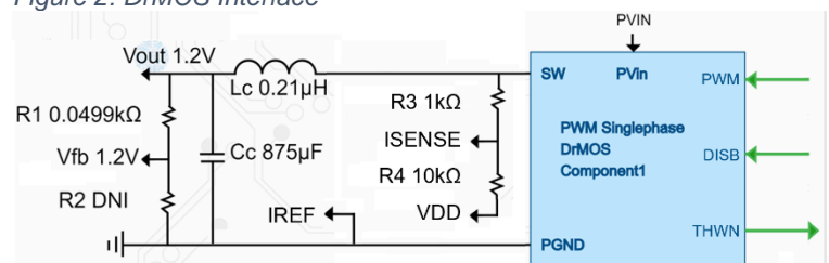
Figure 2: DrMOS Interface
